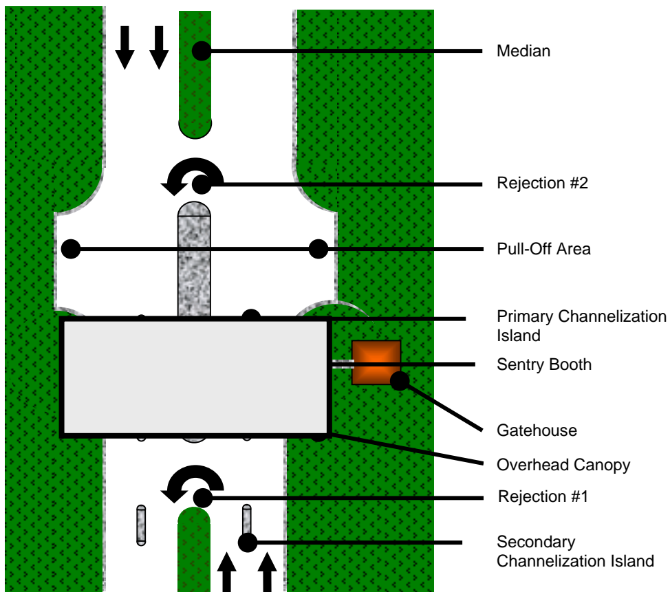
Figure 6-4 Access Control Zone with Single Pull-Off Area for all Inbound Lanes
